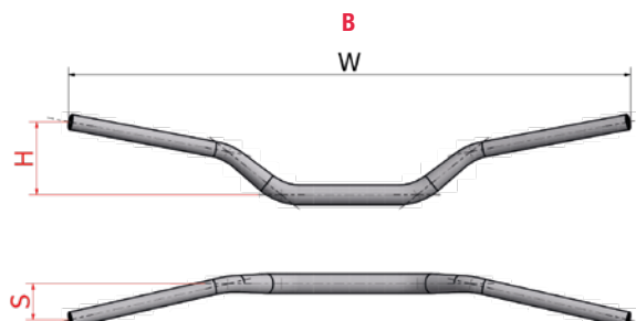
DIMENSIONS (MM)
